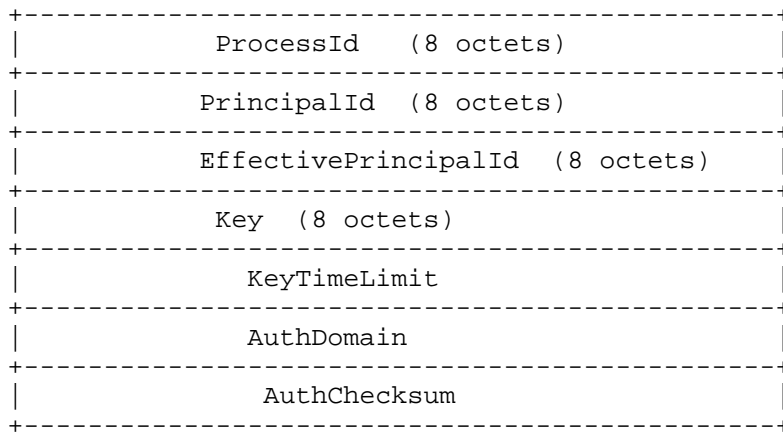
Figure III-1: Authenticator Format
