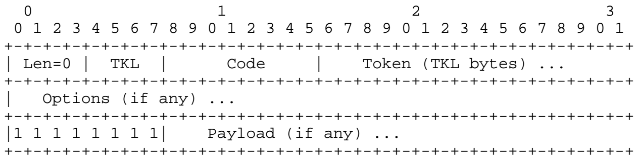
Figure 13: CoAP Message Format over WebSockets
