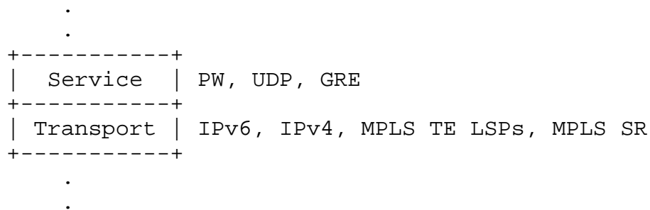
Figure 4: DetNet adaptation to data plane
