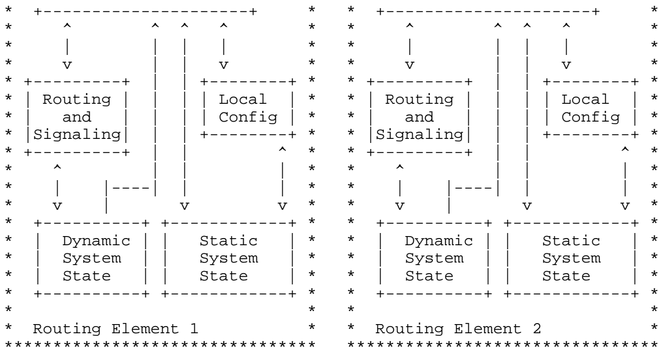
Figure 1: Architecture of I2RS clients and agents
