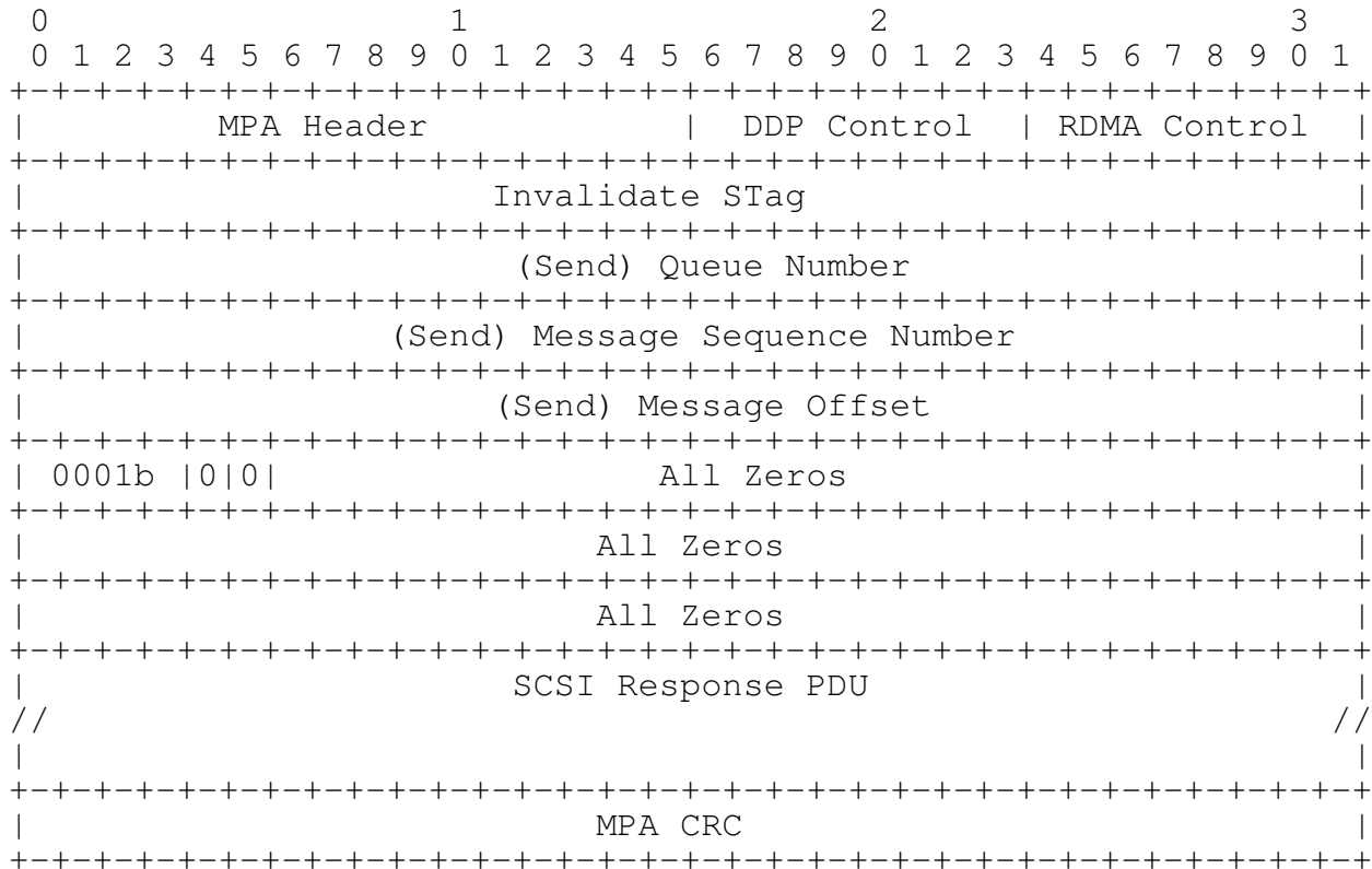
Figure 13 SendInvSE Message containing SCSI Response PDU
