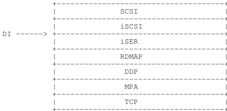
Figure 1 Example of iSCSI/iSER Layering in Full Feature Phase
