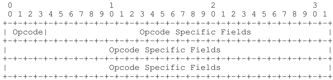
Figure 2 iSER Header Format
