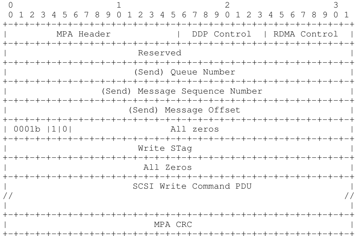
Figure 10 SendSE Message containing a SCSI Write Command PDU
