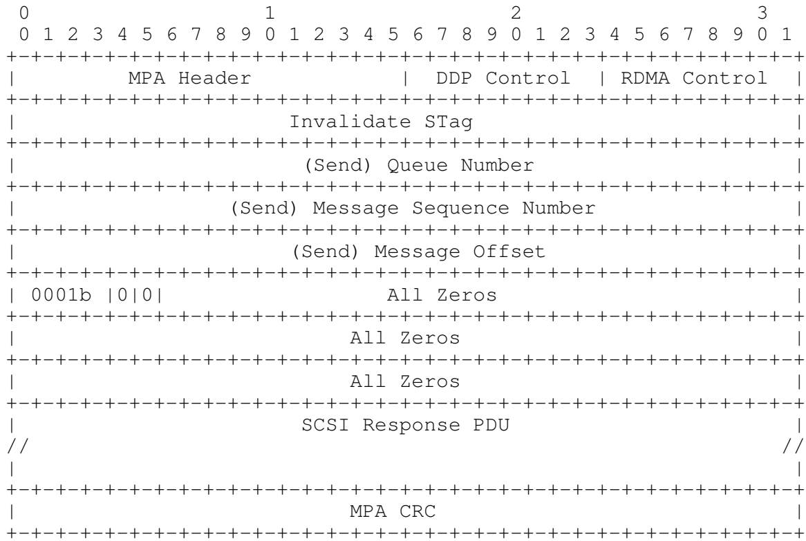
Figure 13 SendInvSE Message containing SCSI Response PDU
