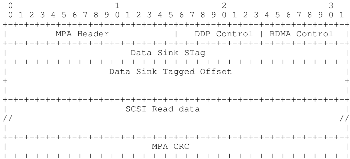
Figure 9 RDMA Write Message containing SCSI Read Data
