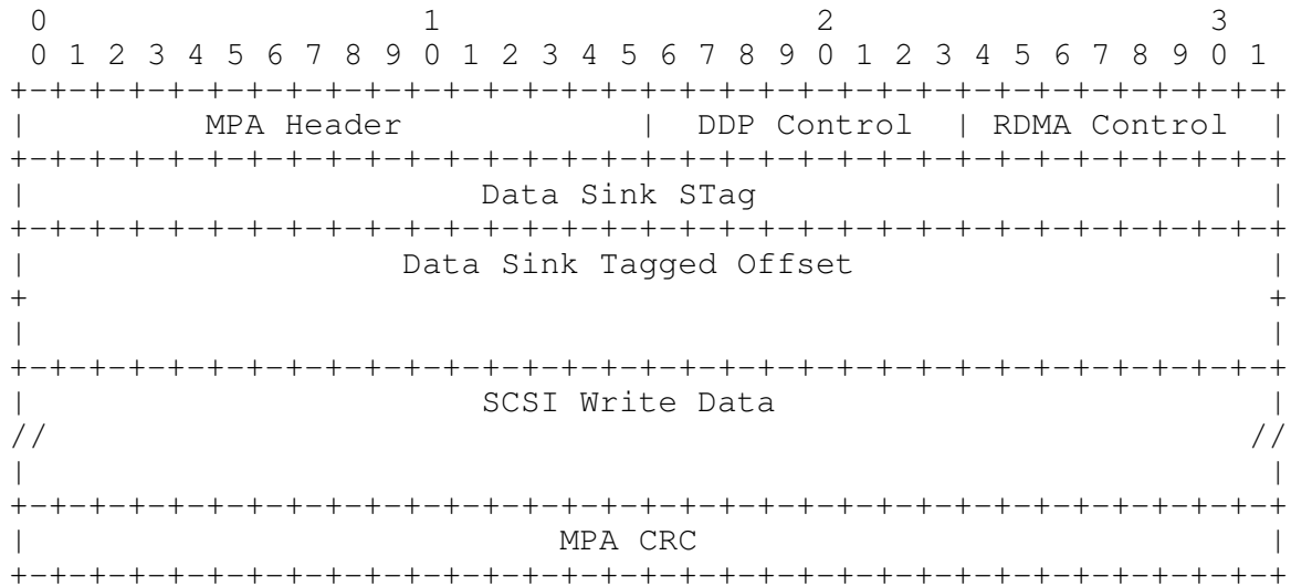
Figure 12 RDMA Read Response Message containing SCSI Write Data
