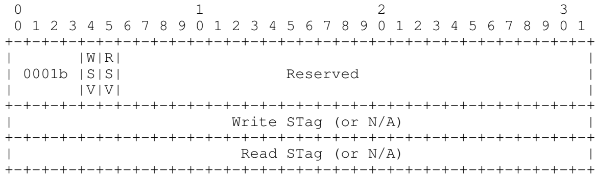
Figure 3 iSER Header Format for iSCSI Control-Type PDU
