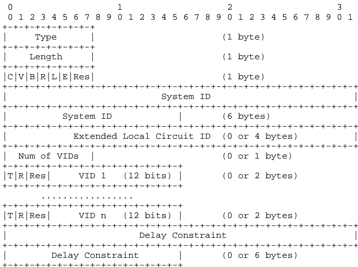
Figure 3: Hop sub-TLV
