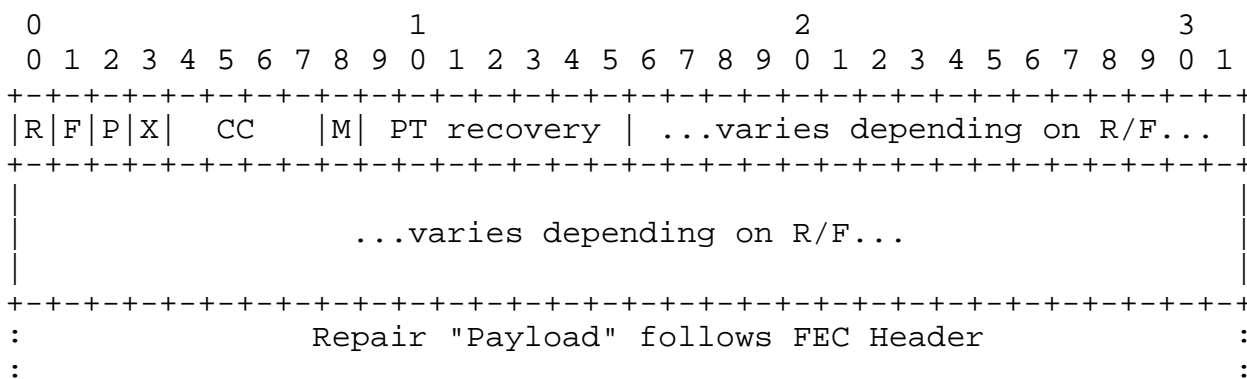
Figure 10: FEC Header
