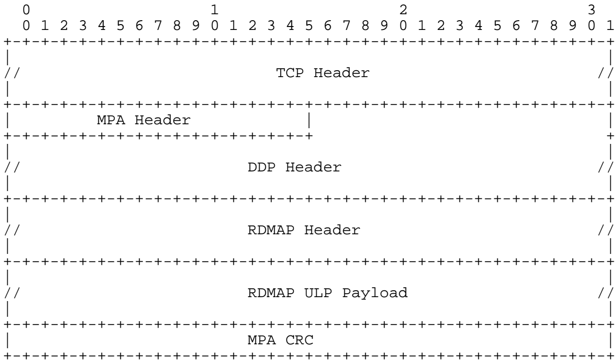
Figure 2 MPA, DDP, and RDMAP Header Alignment
