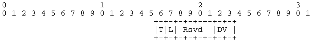
Figure 3 DDP Control Field
