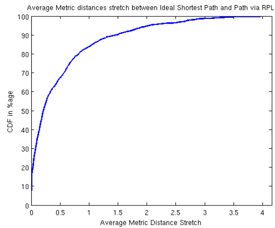
Figure 6: CDF: ETX metric stretch versus ETX value.
