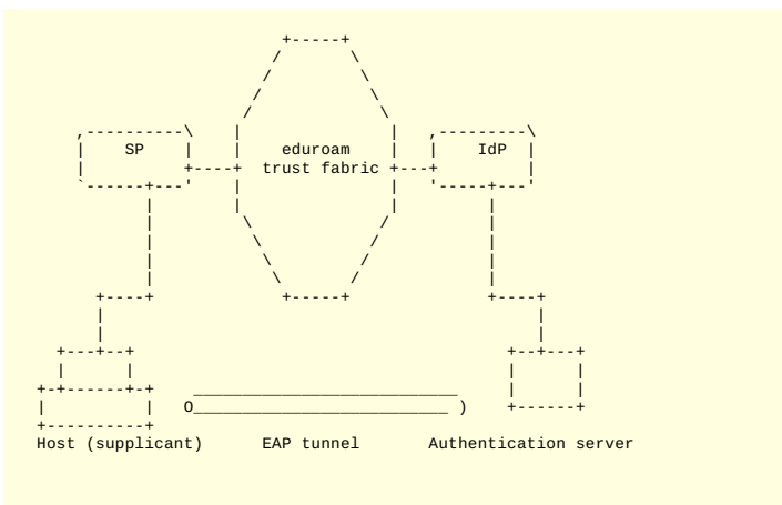
Figure 1: Tunneled EAP
