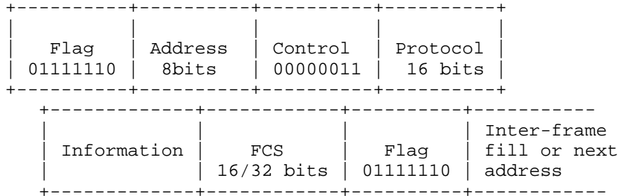
Figure 2. Frame format
