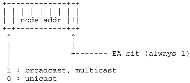
Figure 3 Address format
