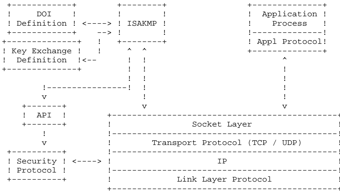
Figure 1: ISAKMP Relationships
