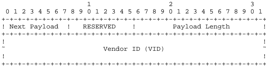
Figure 17: Vendor ID Payload Format
