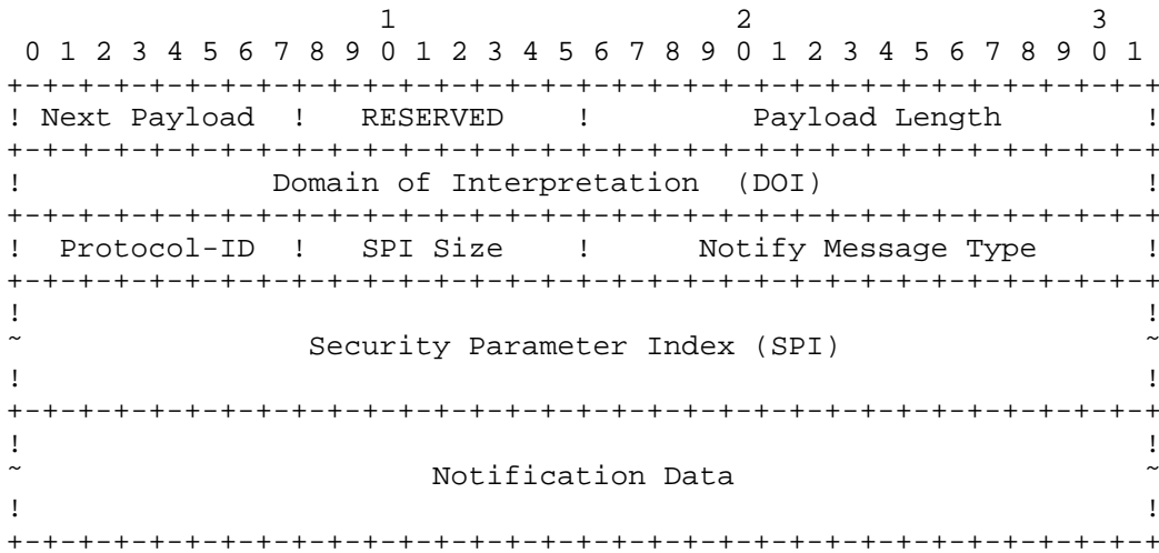
Figure 15: Notification Payload Format
