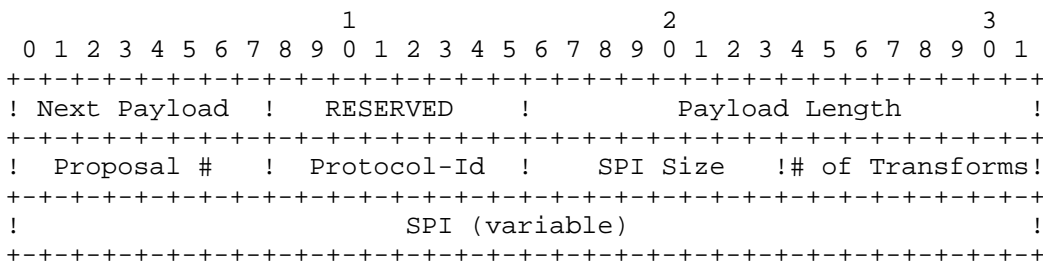
Figure 6: Proposal Payload Format
