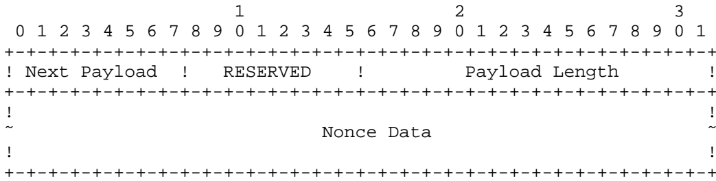
Figure 14: Nonce Payload Format
