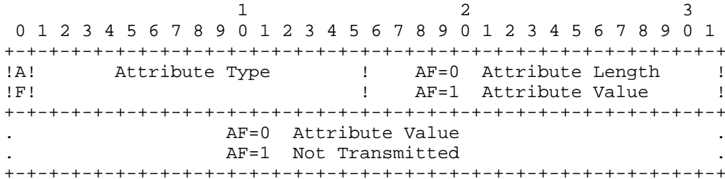
Figure 4: Data Attributes
