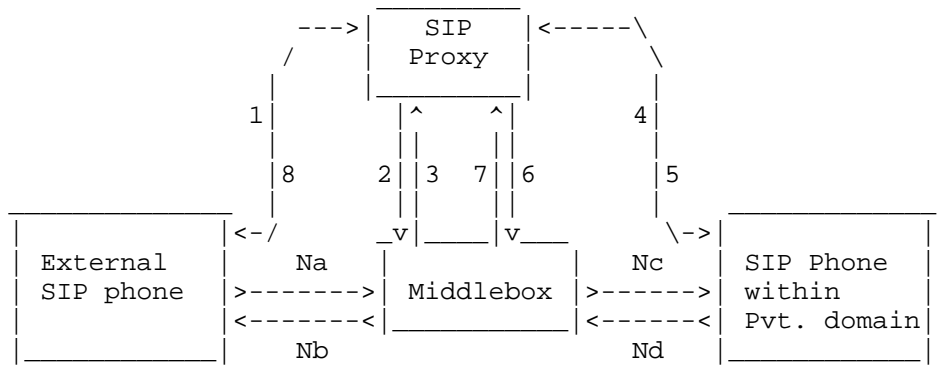
Figure 3: MIDCOM framework illustration with In-Path SIP Proxy
