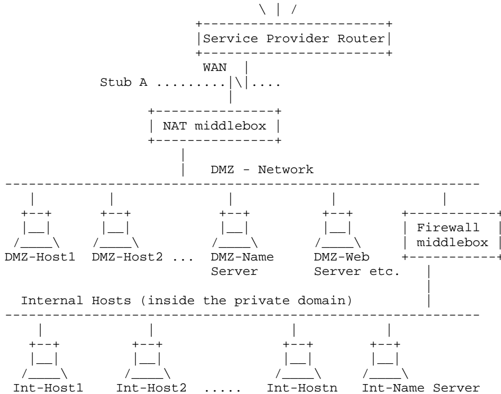
Figure 4: DMZ network configuration of a private domain.
