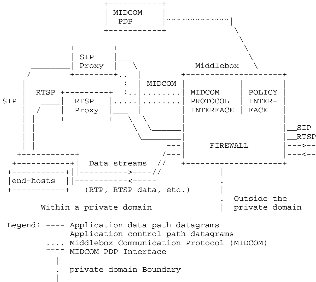
Figure 2: In-Path MIDCOM Agents for middlebox Communication
