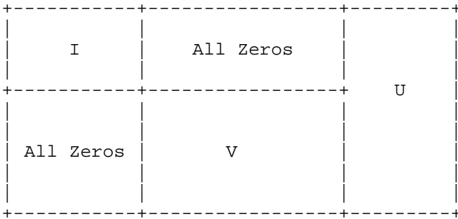
Figure 5: Submatrices of A in the first phase
