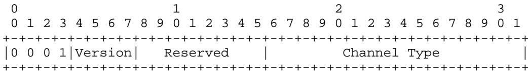
Figure 3: PW Associated Channel Header
