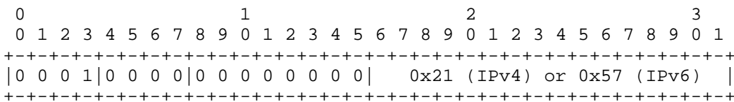
Figure 4: PW Associated Channel Header for VCCV
