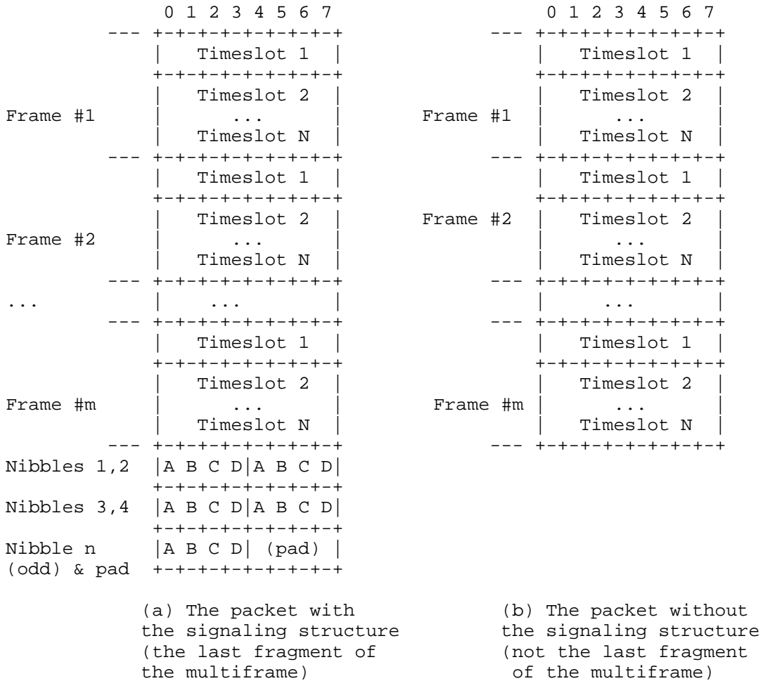
Figure 5. The CESoPSN Packet Payload Format for Trunk-Specific NxDS0 with CAS
