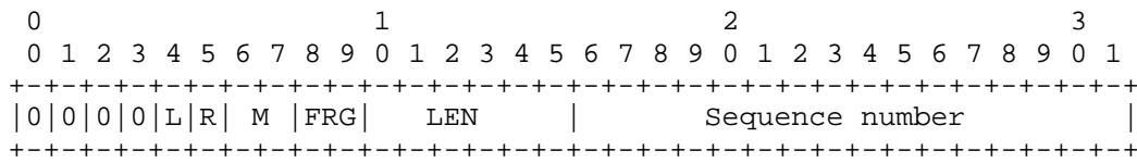
Figure 2. Structure of the CESoPSN Control Word
