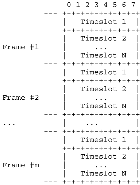
Figure 3. The CESoPSN Packet Payload Format for the Basic NxDS0 Service
