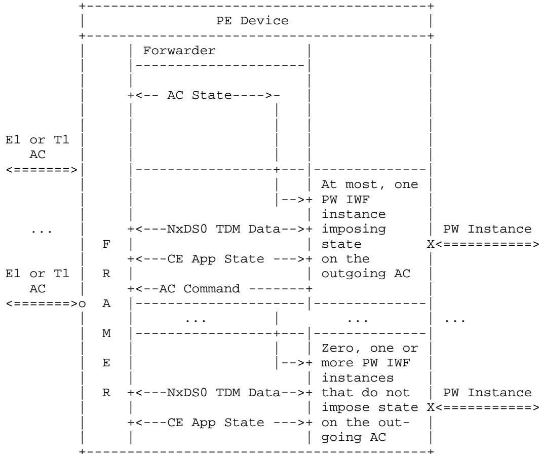
Figure B.1. Reference PE Architecture for NxDS0 Services
