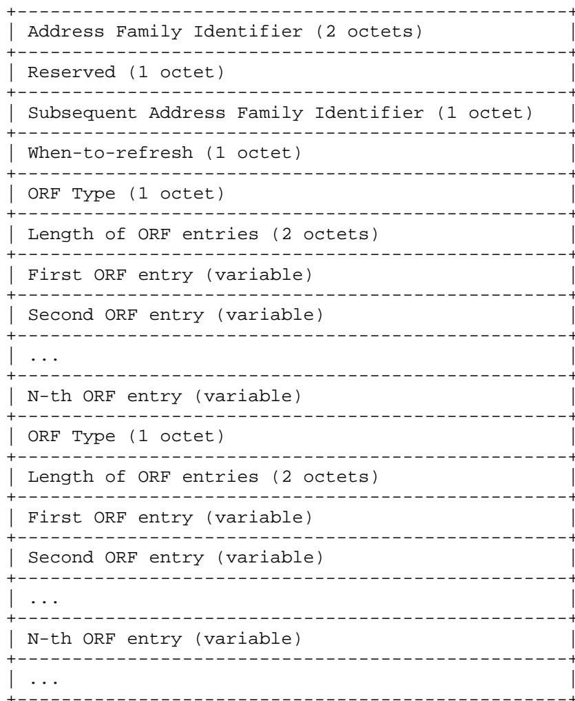
Figure 1: Carrying ORF Entries in the ROUTE-REFRESH Message
