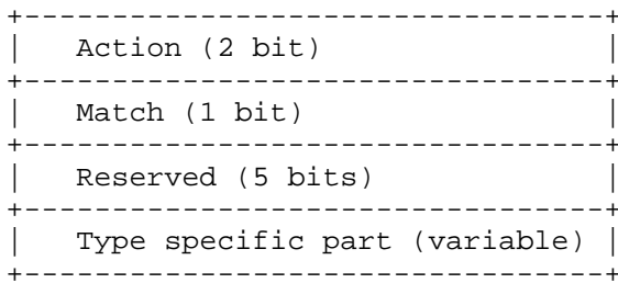
Figure 2: ORF Entry Encoding
