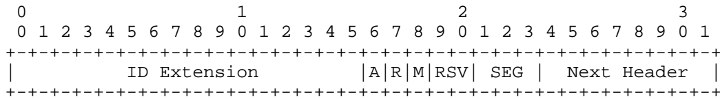
Figure 2: SEAL Header Format
