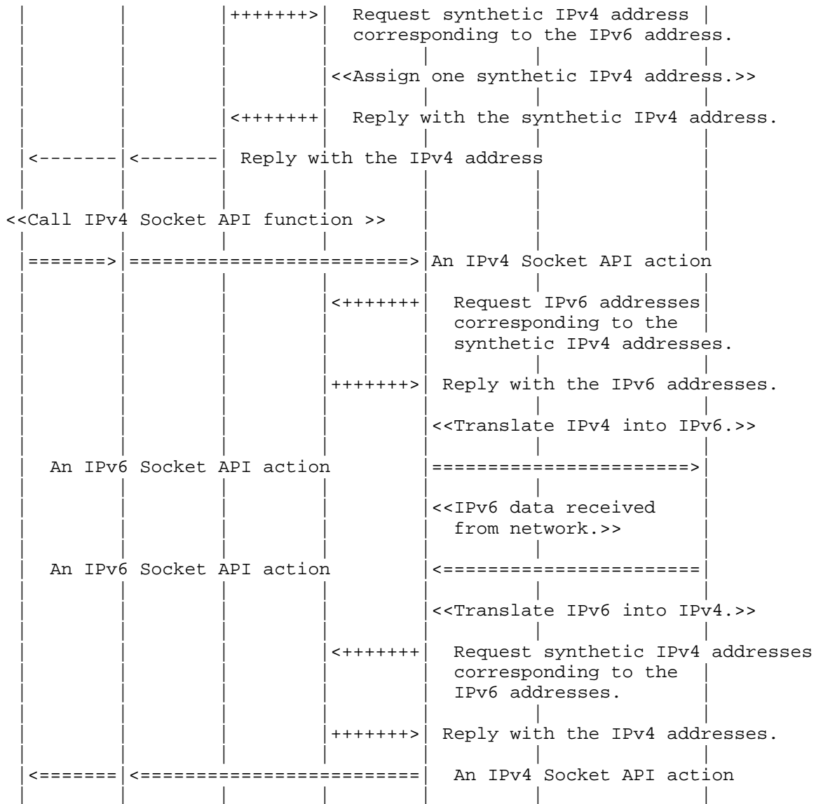
Figure 6: Example of BIH as API Addition
