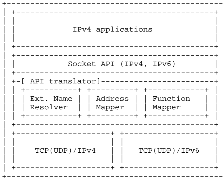
Figure 1: Architecture of a dual-stack host using protocol translation at the socket layer
