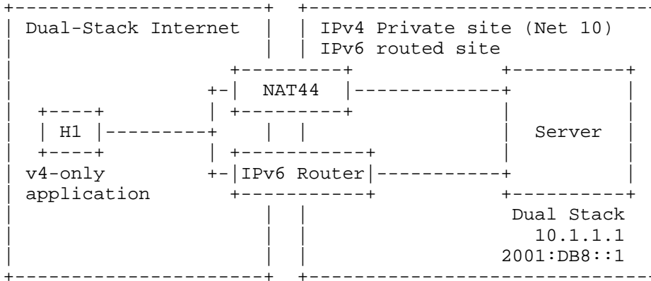
Figure 5: Network Scenario #2
