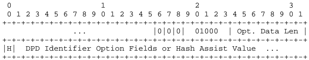
Figure 2: IPv6 SMF_DPD Hop-by-Hop Option Header
