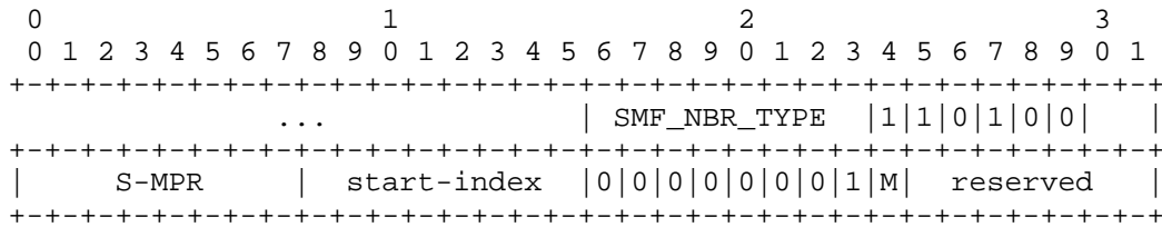
Figure 10: S-MPR Address Block TLV Example
