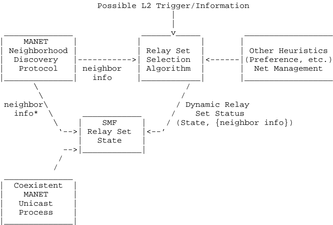
Figure 5: SMF Reduced Relay Set Information Flow
