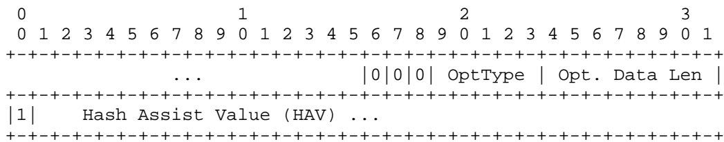
Figure 4: IPv6 SMF_DPD Option Header in H-DPD Mode
