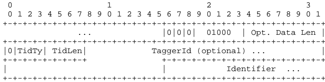
Figure 3: IPv6 SMF_DPD Option Header in I-DPD mode
