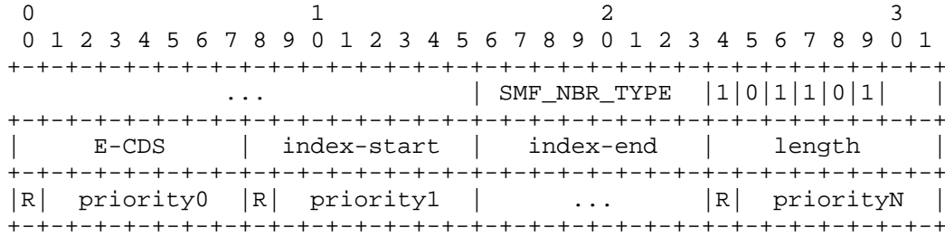
Figure 8: E-CDS Address Block TLV Example 2
