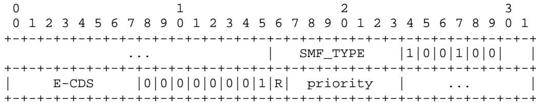
Figure 6: E-CDS Message TLV Example
