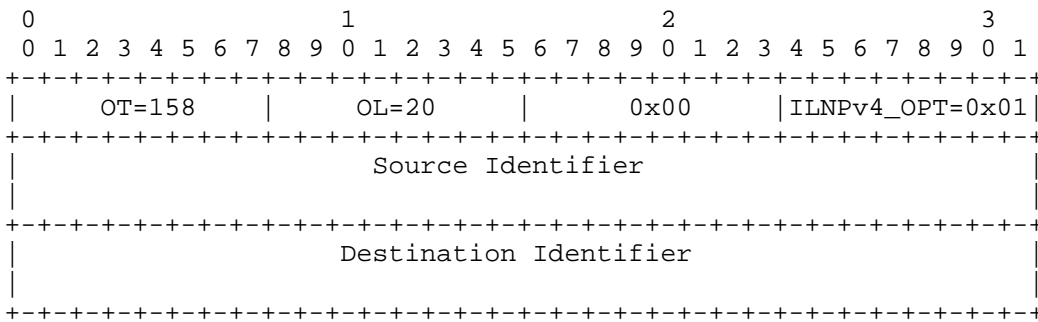
Figure 2: ILNP Identifier Option for IPv4
