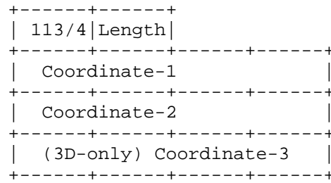
Figure 4: Point Encoding
