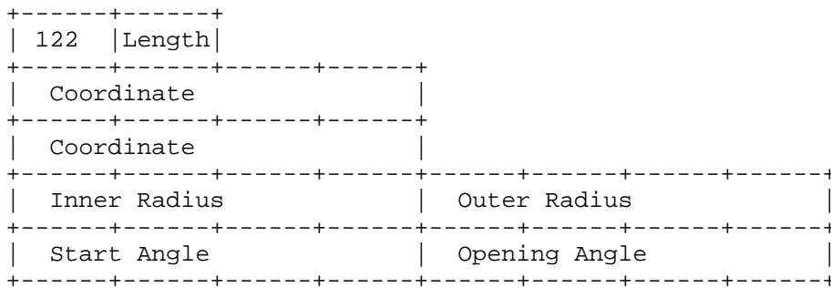
Figure 15: Arc-Band Encoding
