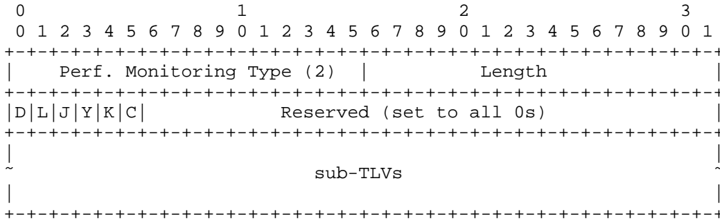
Figure 7: Performance Monitoring Sub-TLV Format
