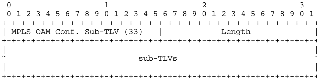
Figure 1: MPLS OAM Configuration Sub-TLV Format
