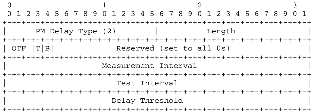
Figure 9: MPLS OAM PM Delay Sub-TLV Format
