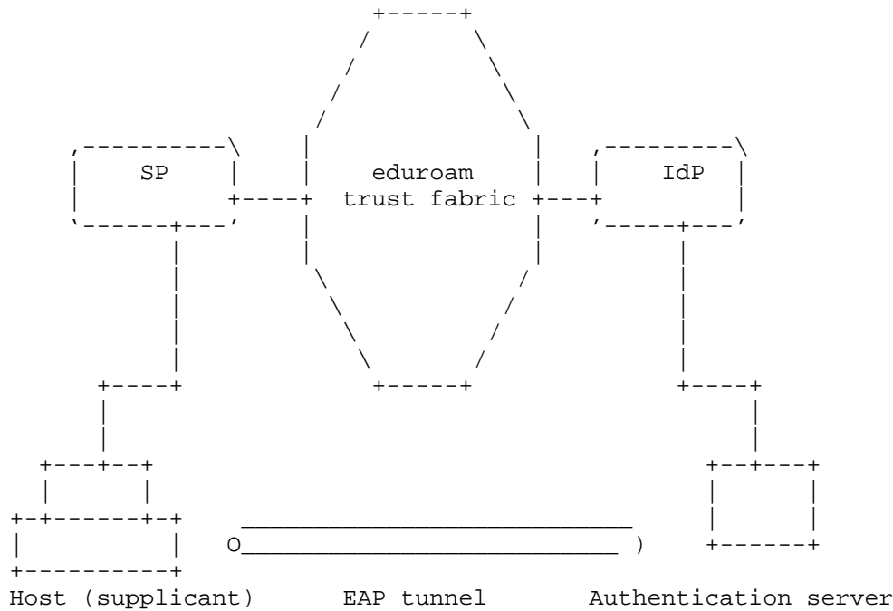
Figure 1: Tunnelled EAP
