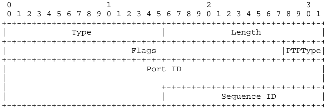
Figure 2: PTP Sub-TLV Format
