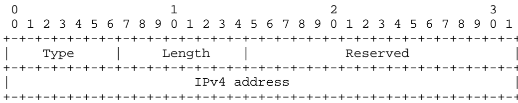
Figure 8: IPv4 Sub-TLV Format
