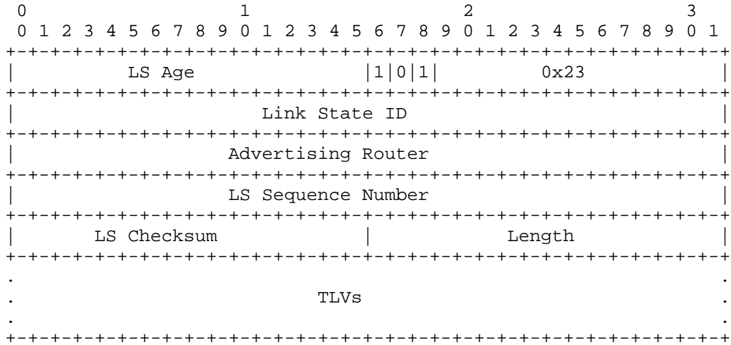
E-Inter-Area-Prefix-LSA
