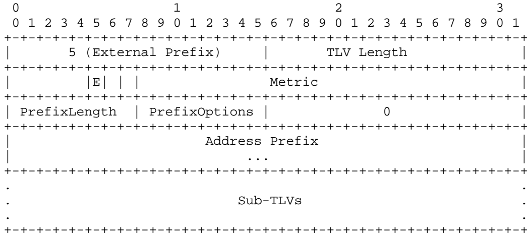
External-Prefix TLV
