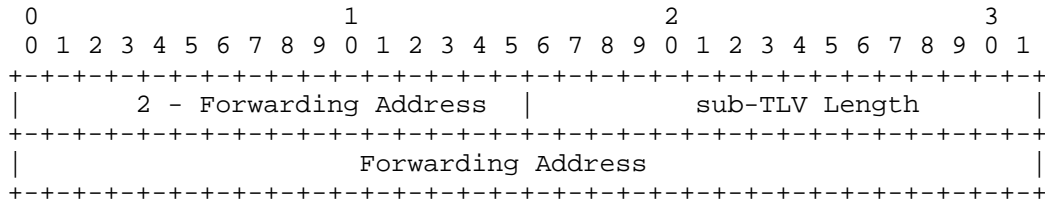
IPv4-Forwarding-Address TLV
