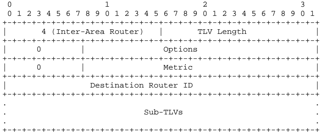
Inter-Area-Router TLV
