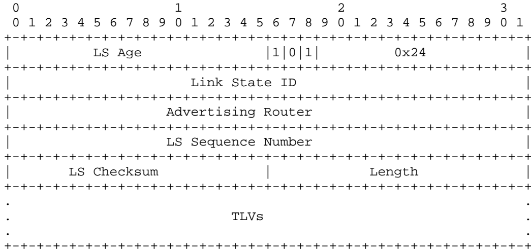
E-Inter-Area-Router-LSA
