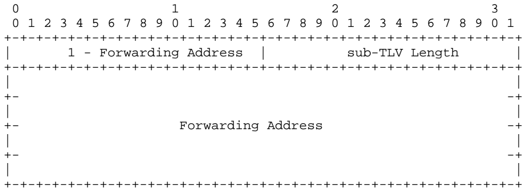
IPv6-Forwarding-Address TLV
