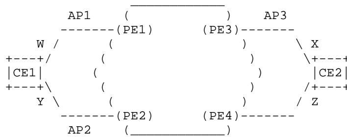
Figure 16: Dual-Homing Scenario
