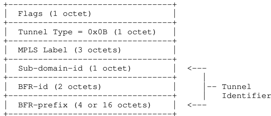
Figure 1: PMSI Tunnel Attribute for BIER
