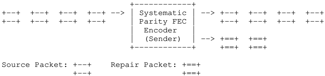
Figure 1: Block Diagram for Systematic Parity FEC Encoder
