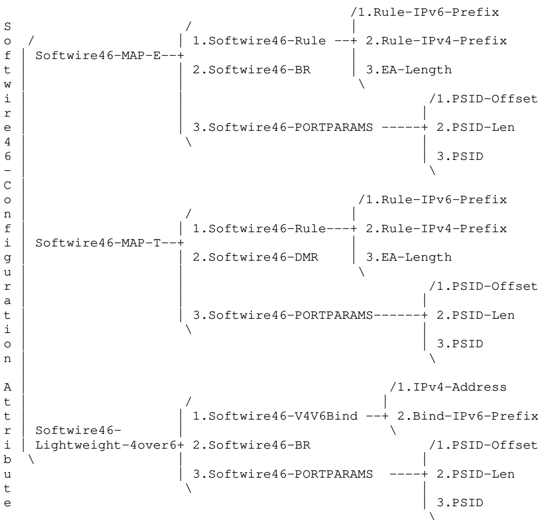
Figure 1: Software46 Attribute Hierarchy
