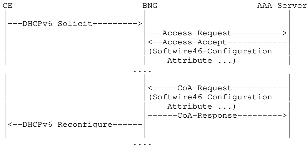
Figure 3: Change of Configuration Example
