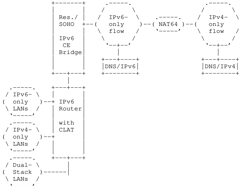
Figure 18: CE Setup with Bridged CLAT, without DNS64
