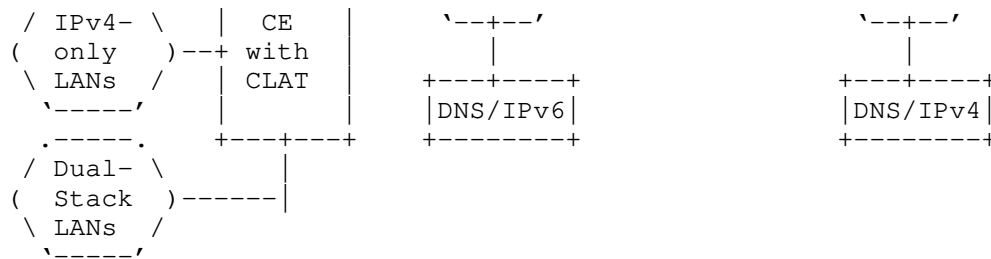
Figure 17: CE Setup with Built-In CLAT, without DNS64
