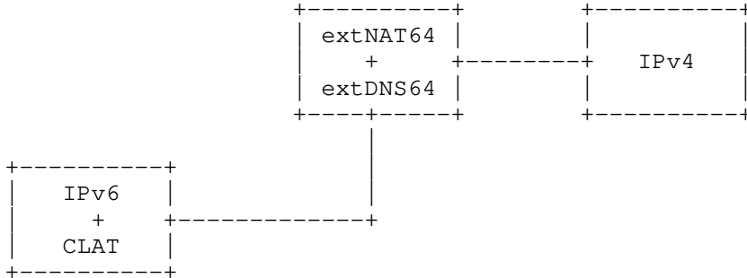
Figure 7: 464XLAT with DNS64; NAT64 and DNS64 in an External Provider
