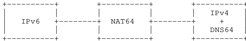
Figure 12: NAT64; DNS64 in IPv4-Only Hosts
