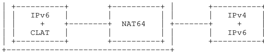
Figure 14: DS Enterprise with CLAT, DS Internet, without DNS64
