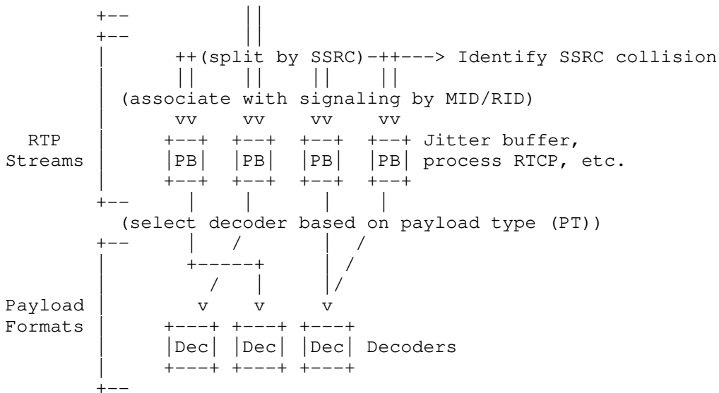
Figure 1: RTP Demultiplexing Process
