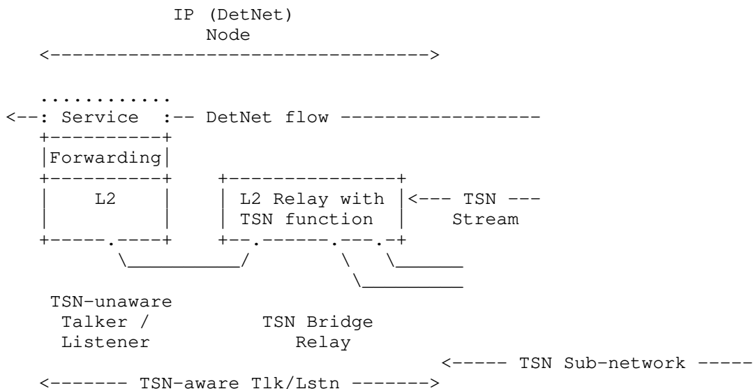
Figure 2: IP (DetNet) Node with TSN Functions
