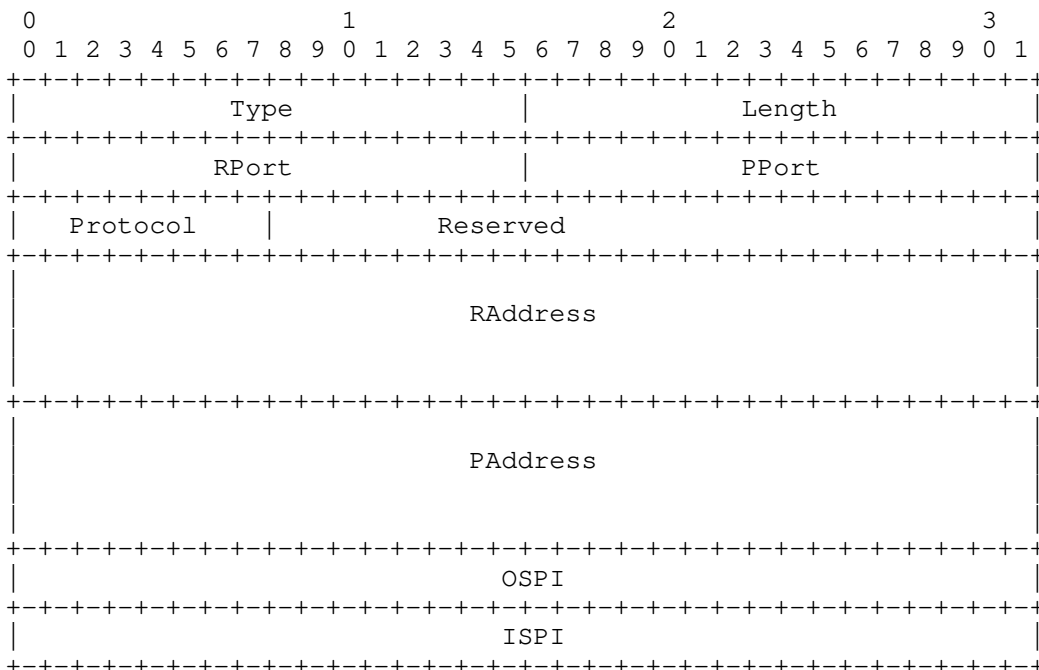
Figure 13: Format of the PEER_PERMISSION Parameter
