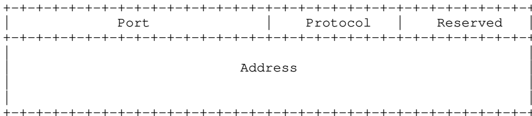
Figure 12: Format of the RELAYED_ADDRESS and MAPPED_ADDRESS Parameters
