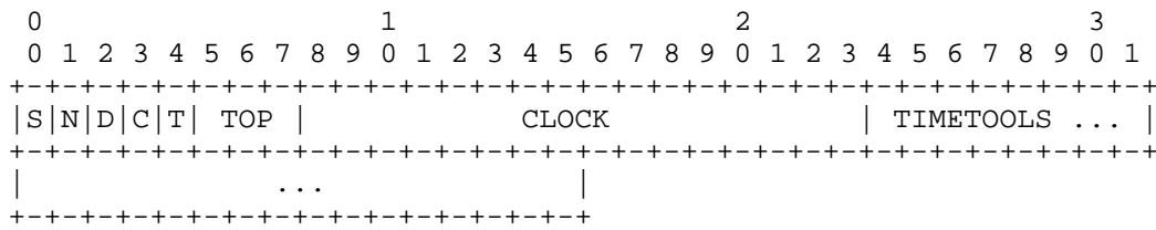
Figure B.3.1 -- System Chapter Q Format
