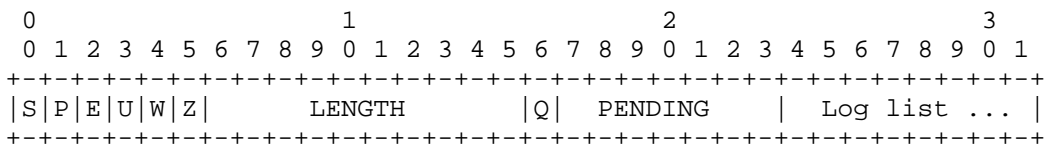
Figure A.4.1 -- Top-Level Chapter M Format
