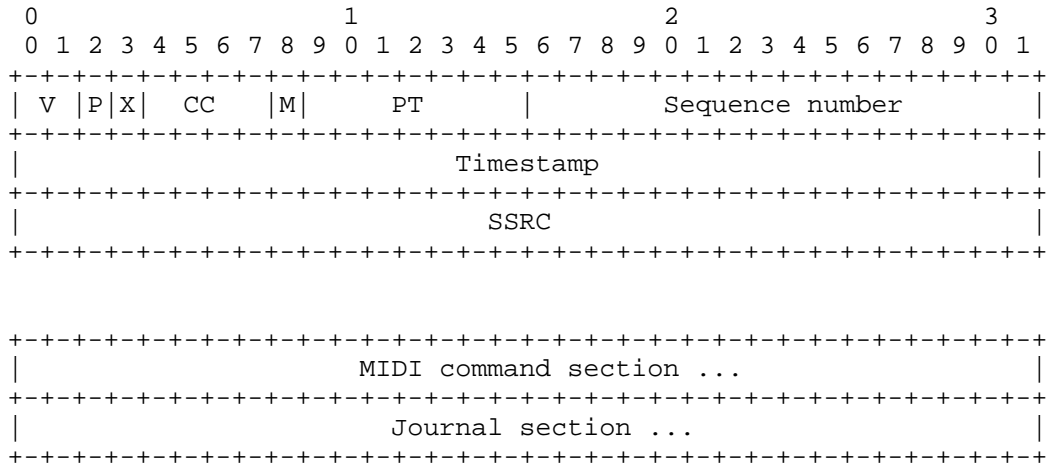
Figure 1 -- Packet Format
