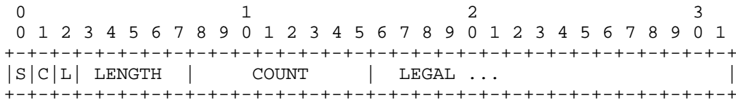
Figure B.1.5 -- Undefined System Real-Time Command Log Format
