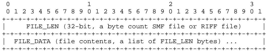
Figure E.5 -- The FILE_BLK Field Format
