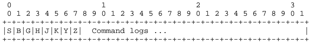
Figure B.1.1 -- System Chapter D Format
