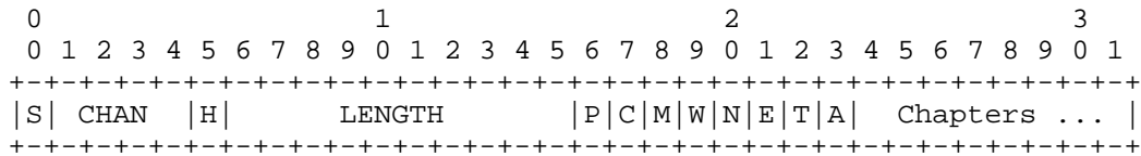
Figure 9 -- Channel Journal Format
