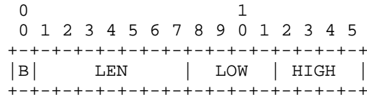
Figure A.6.2 -- Chapter N Header
