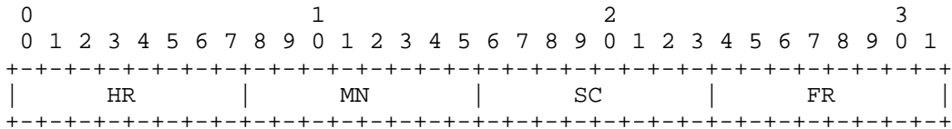
Figure B.4.3 -- COMPLETE Field Format, Q = 0
