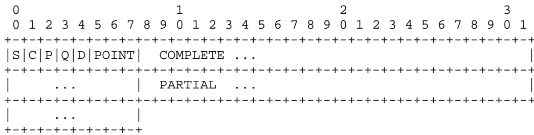
Figure B.4.1 -- System Chapter F Format
