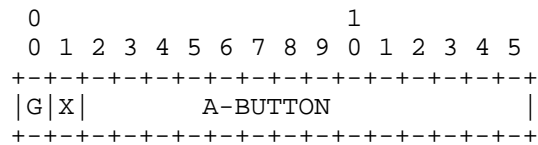
Figure A.4.5 -- A-BUTTON Field
