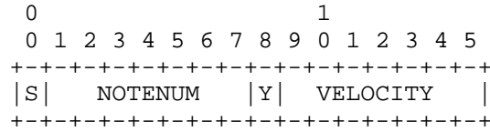
Figure A.6.3 -- Chapter N Note Log
