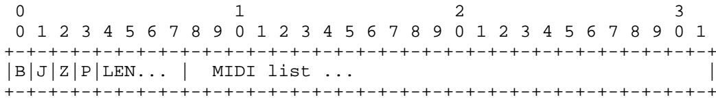
Figure 2 -- MIDI Command Section
