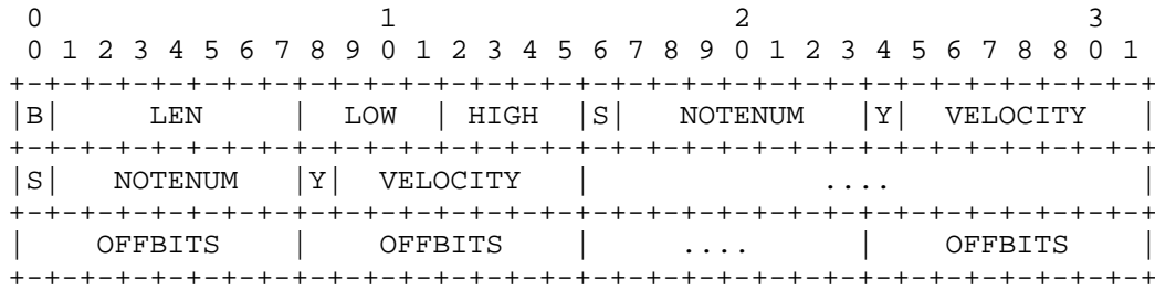
Figure A.6.1 -- Chapter N Format
